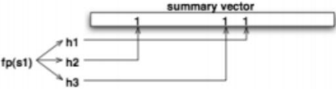
(a) Inserting segment s1 to the Summary Vector
