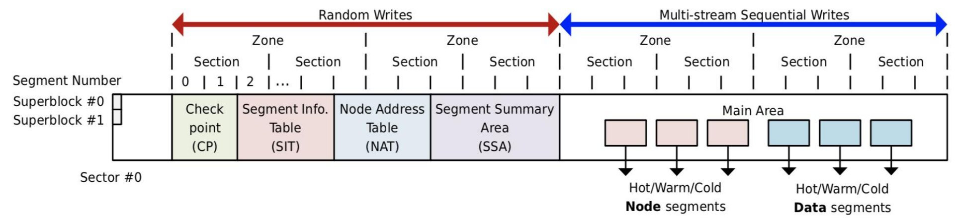
Figure 1: On-disk layout of F2FS.
