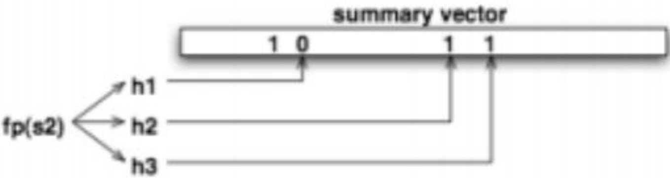
(b) Looking up segment s2 in the Summary Vector
